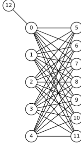
Figure 10: Example for m = 5, n = 7 . Vertex 12 is a , vertex 0 is b , vertices 5 through 11 compose set C , and vertices 1 through 4 compose set D .
