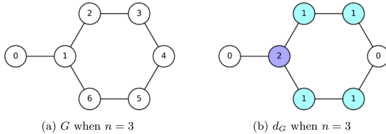
Figure 9: G and d_G when n = 3
