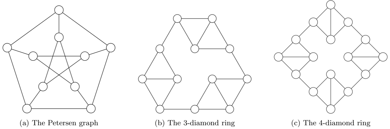
Figure 4: The Petersen graph and the n -diamond ring for n = 3, 4
