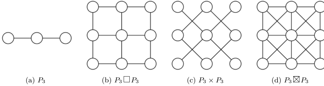
Figure 11: The Cartesian, tensor, and strong products between two copies of P_3
