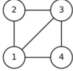
Figure 5: The Diamond Graph
