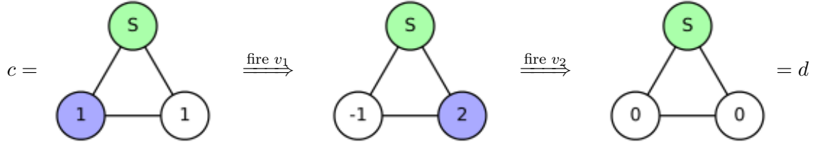
Figure 2: Equivalence of the recurrent identity and the all-zero configuration
