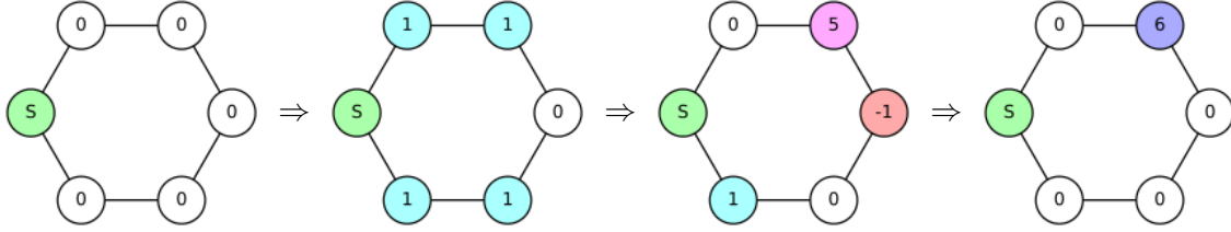
Figure 8: Example firing process for C_6
