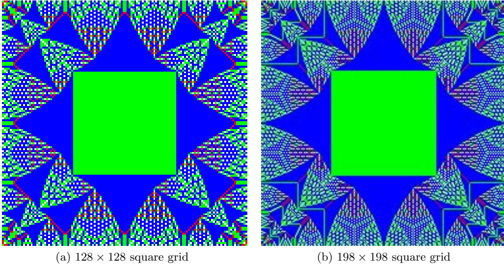
Figure 3: The recurrent identity of the 128 \times 128 and 198 \times 198 square grids, as shown in [15]. 0, 1, 2, and 3 chips are displayed as orange, red, green, and blue, respectively.
