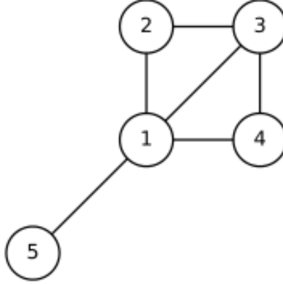
Figure 6: The Diamond Graph with a tree of size 1 added to vertex v_1
