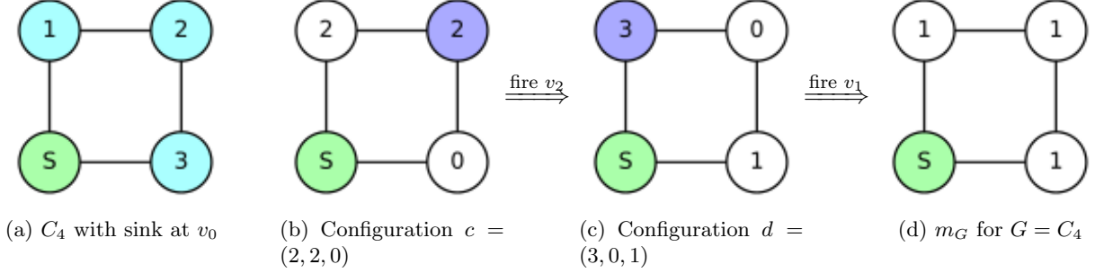
Figure 1: Chip-firing on C_4
