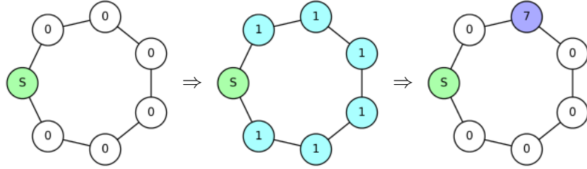
Figure 7: Example firing process for C_7
